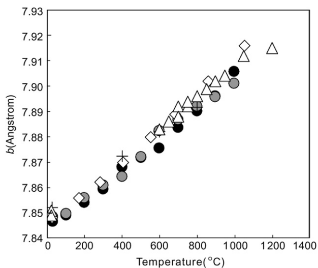
Figure 4 Variation of b -axis of kyanite with temperature. See the caption of Fig. 3 for the symbol information and datum sources. For most data, error bars are smaller than or equal to symbol size.
