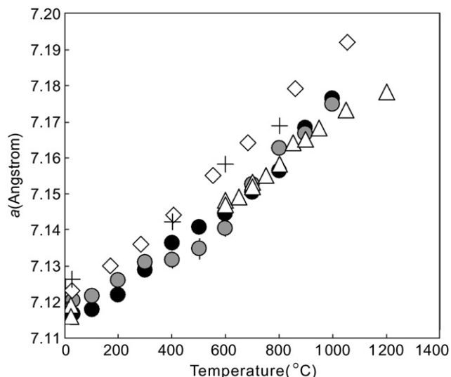
Figure 3 Variation of a -axis of kyanite with temperature. Solid circles, data collected at different temperatures in the 1st series of experiments; shaded circles, data collected at different temperatures in the 2nd series of experiments; empty triangles, data from Gatta et al. (2006); pluses, data from Winter and Ghose (1979); diamonds, data from Skinner et al. (1961). For most data, error bars are smaller than or equal to symbol size.
