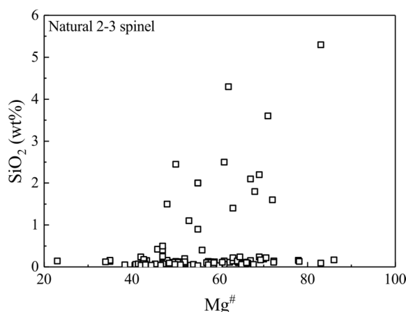
Figure 1. \text{SiO}_2 (wt %) vs. \text{Mg}^\# of some natural 2-3 spinels. \text{Mg}^\# , 100 \text{ Mg}/(\text{Mg} + \text{Fe}) in molar ratio. Data sources are Sigurdsson et al. [65], Sobolev & Nikogosian [66], Kamenetsky et al. [67], Franz & Wirth [68], and Chistyakova et al. [69].
